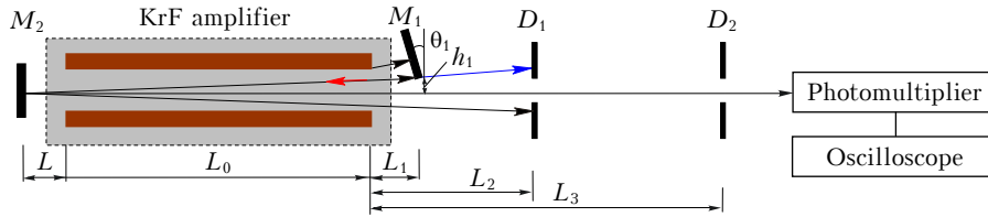
Fig. 1. The experimental schematic
