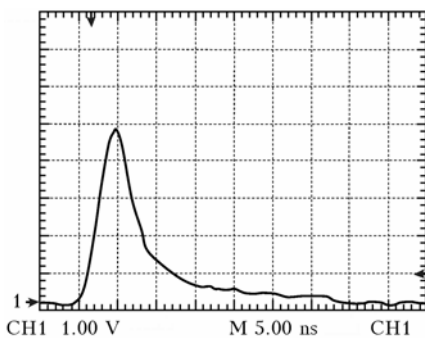
Fig. 6. The compressed ASE pulse waveform
