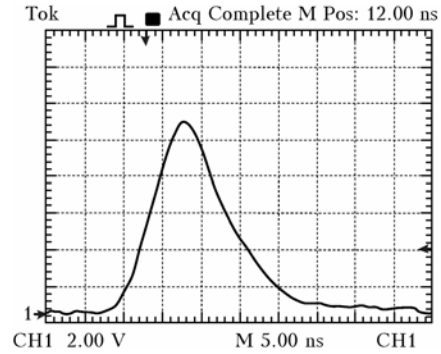
Fig. 2. Waveform before compression
