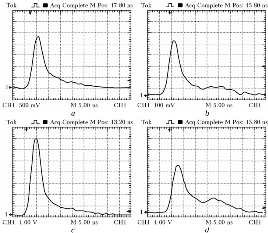
Fig. 3. The ASE pulse waveform \theta for different values of pulse compression
