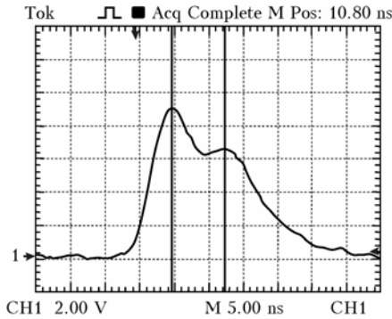
Fig. 5. The compressed ASE pulse waveform
