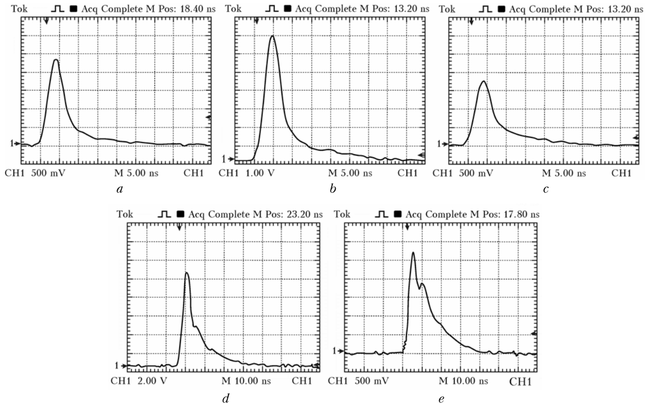
Fig. 4. The ASE pulse waveform r_1 for different values of pulse compression
