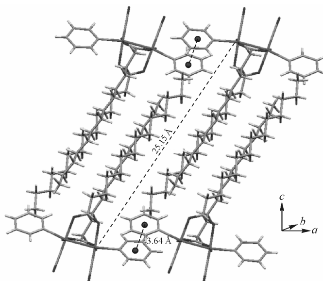
Fig. 4. Main interactions involved in the crystalline packing of 5a , π-stacking interactions between adjacent pyridyl groups and van der Waals interactions between parallel alkyl chains
