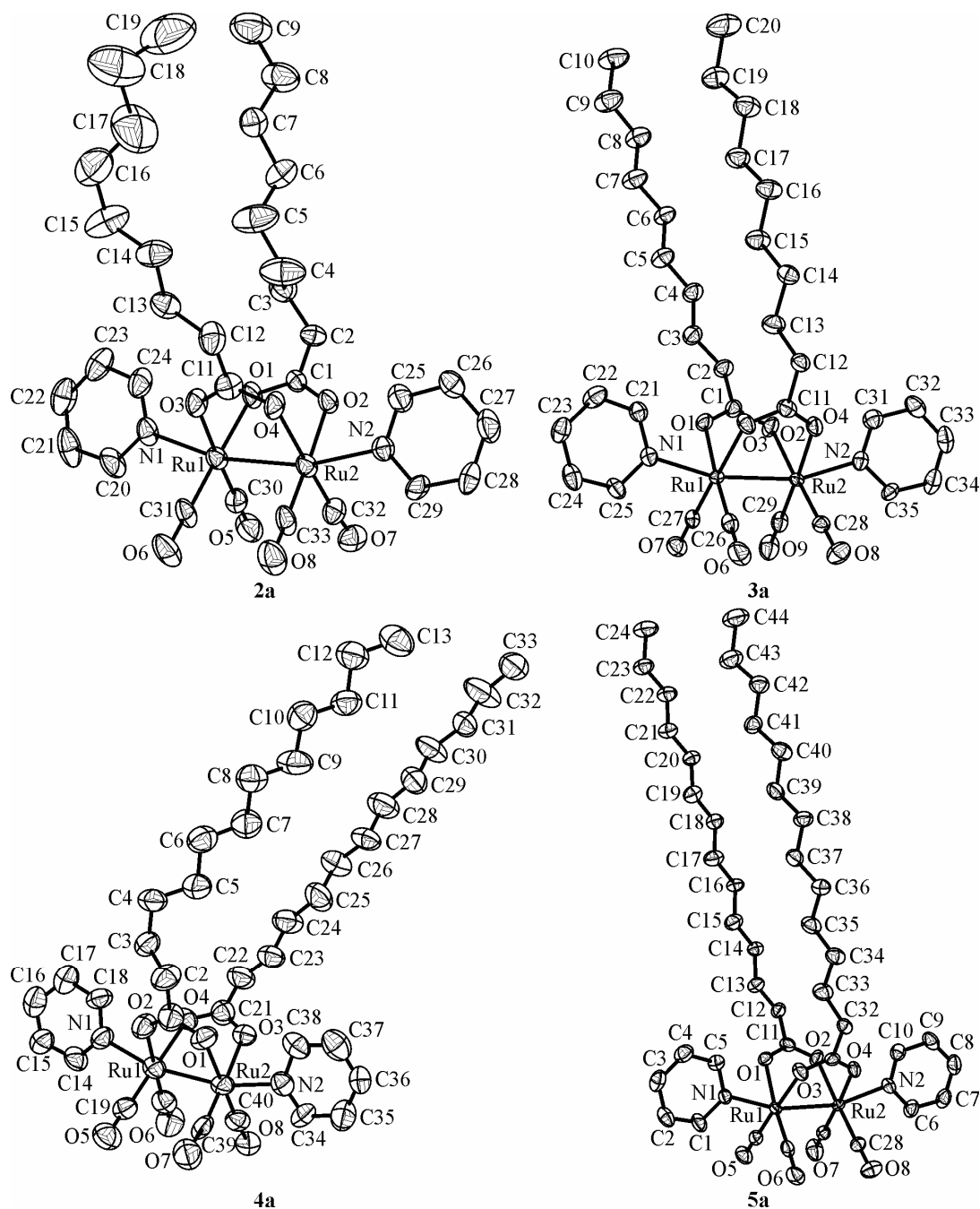
Fig. 2. ORTEP drawings of Ru 2 (CO) 4 {OOC(CH 2 ) 7 CH 3 } 2 (C 5 H 5 N) 2 ( 2a ), Ru 2 (CO) 4 {OOC(CH 2 ) 8 CH 3 } 2 (C 5 H 5 N) 2 ( 3a ), Ru 2 (CO) 4 {OOC(CH 2 ) 11 CH 3 } 2 (C 5 H 5 N) 2 ( 4a ) and Ru 2 (CO) 4 {OOC(CH 2 ) 12 CH 3 } 2 (C 5 H 5 N) 2 ( 5a ) at 50 % probability level ellipsoids with hydrogen atoms omitted for clarity
