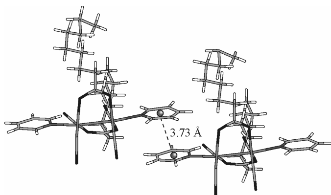
Fig. 3. Parallel \pi -stacking interaction observed in the crystalline packing of 2a
