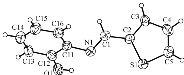
Fig. 1. ORTEP drawing of ImineOH with displacement ellipsoids plotted at a 40 % probability level
