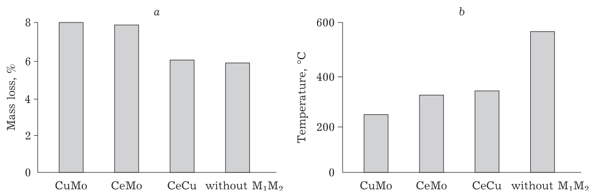
Fig. 5. Effect of precursor nature on the oxidation/decomposition of the support during thermal treatment (in N 2 ) of dried M 1 M 2 O x /Taunite samples: mass loss (a) and the temperature of the start of CO 2 evolution (b).
