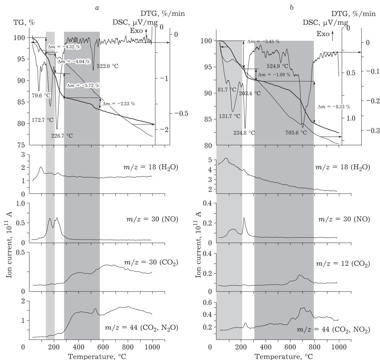
Fig. 4. TG, DTG, DSC and MS curves for samples: CeCu/Taunite (Ce/Cu = 1 : 1) (a) and CuMo/Taunite (Cu/Mo = 1 : 1) (b).
