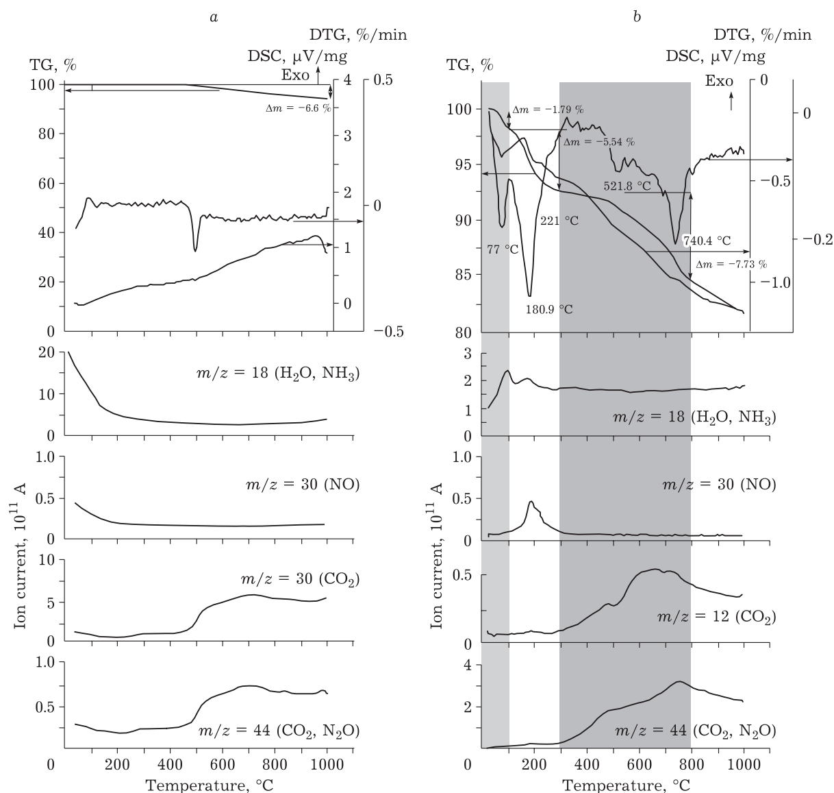
Fig. 3. TG, DTG, DSC and MS curves for samples: Taunite [9] (a) and CeMo/Taunite (Ce/Mo = 1 : 1) (b).
