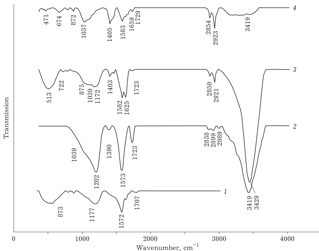
Fig. 2. FTIR spectra of samples: Taunite (1), Taunite-1 (2), CeCu/Taunite-1 (3), CeCu/Taunite (4).
